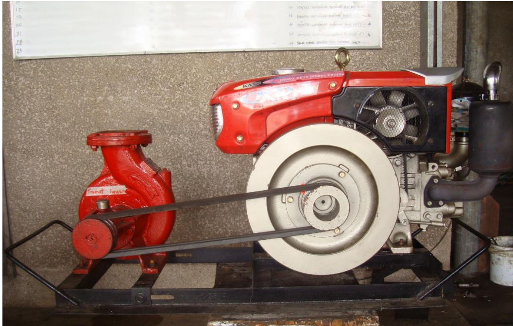
Figure 2. KATO KC40 Centrifugal Pump coupled to a KATO KD120-N Diesel Engine
