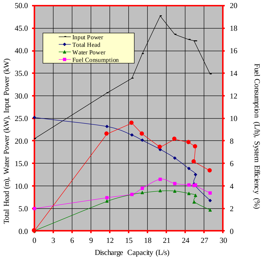
Figure 3. Performance characteristic curves of the KATO KC40 centrifugal pump coupled to KATO KD120-N diesel engine
