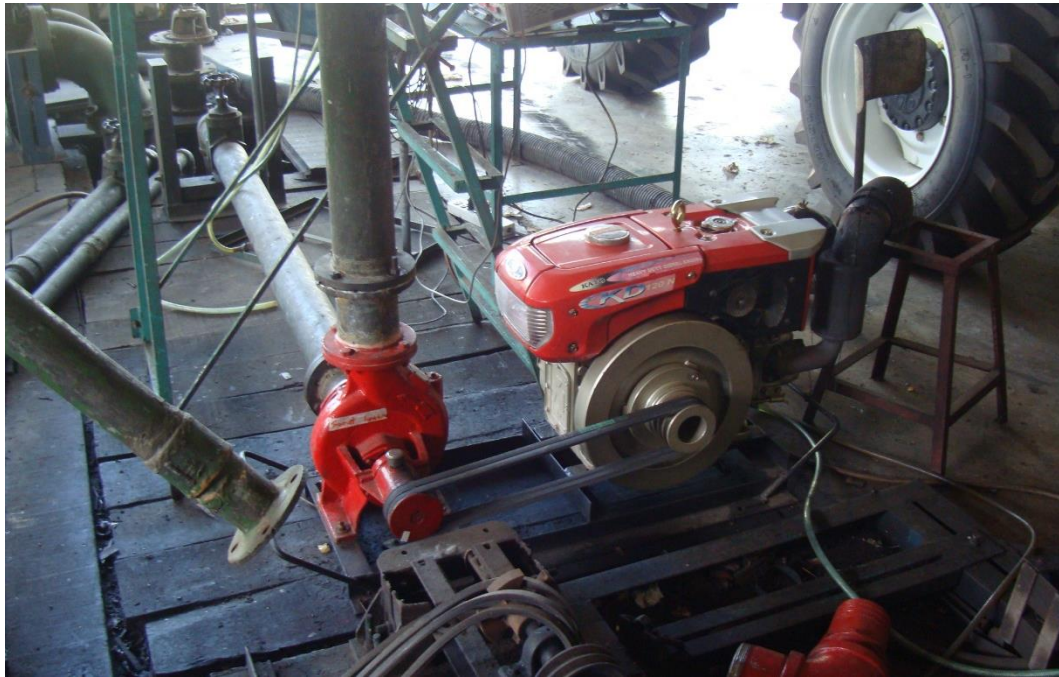
Figure 1. KATO KC40 Centrifugal pump coupled to KATO KD120-N Diesel Engine on the test set-up
